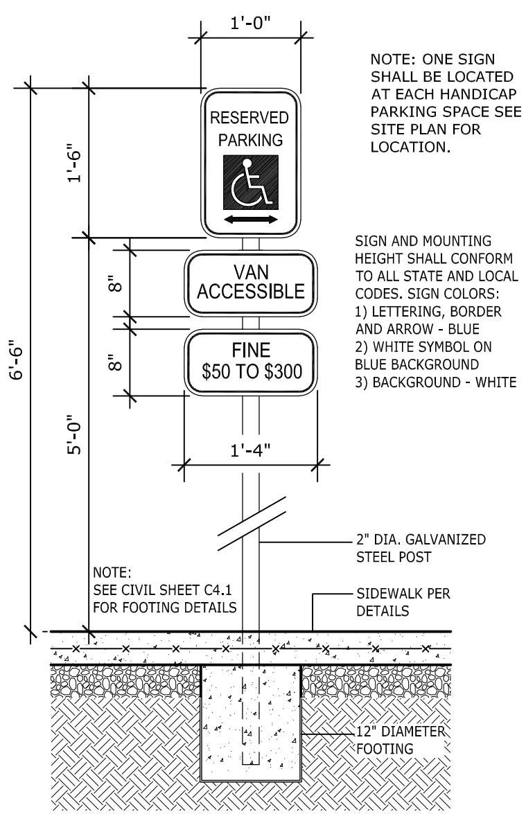
1P H.C. SIGN DETAIL AS102 scale: 3/4" = 1'-0"
