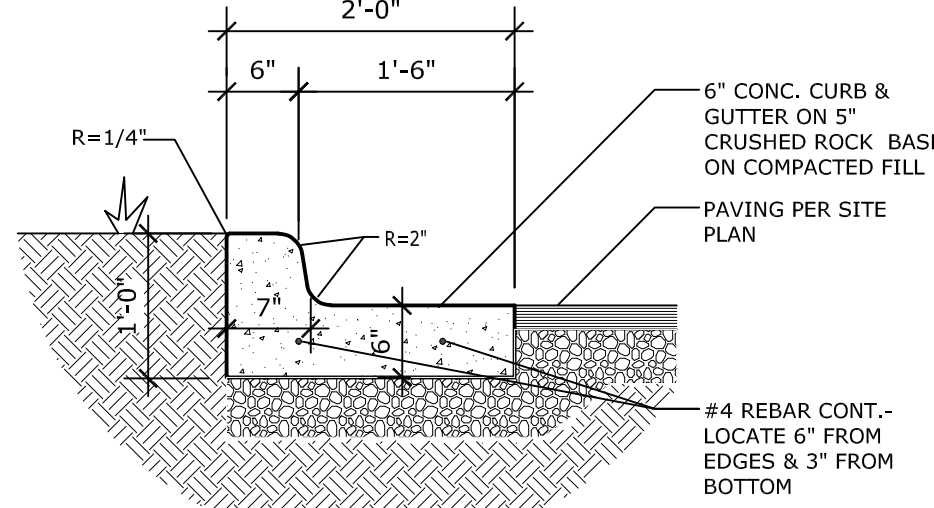
10L CURB/GUTTER DETAIL AS102 scale: 3/4" = 1'-0"
