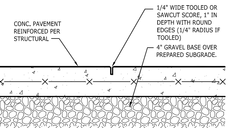
4L CONTROL JOINT AS102 scale: 1-1/2" = 1'-0"
