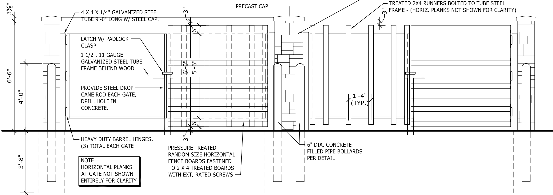
1H TRASH ENCLOSURE ELEVATION AS102 scale: 3/8" = 1'-0"
