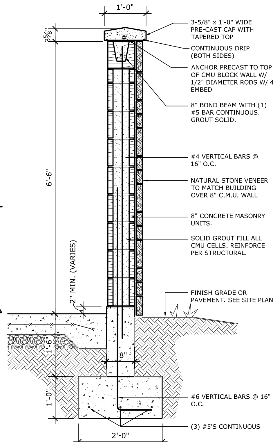
7H WALL SECTION
