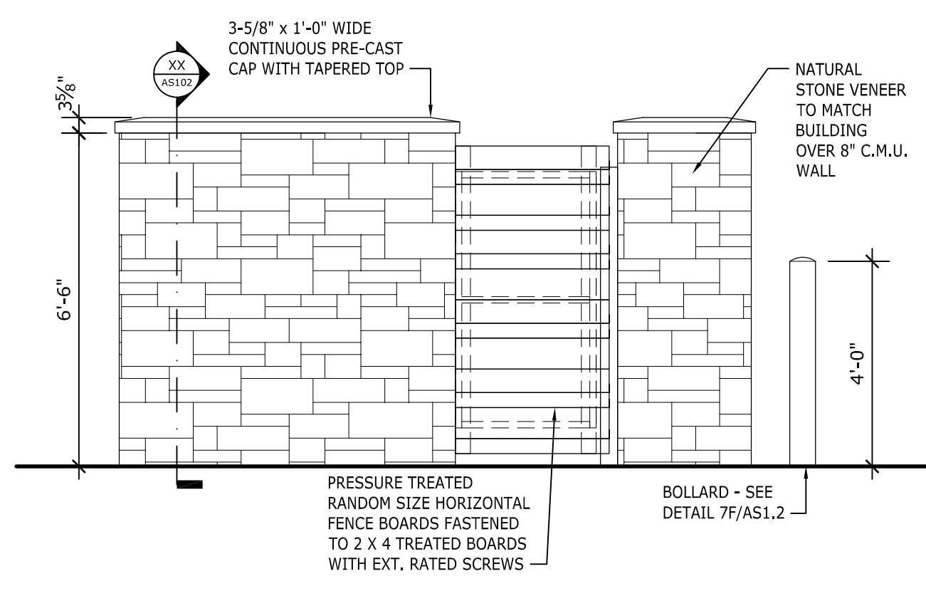
4H TRASH ENCLOSURE ELEVATION AS102 scale: 3/8" = 1'-0"
