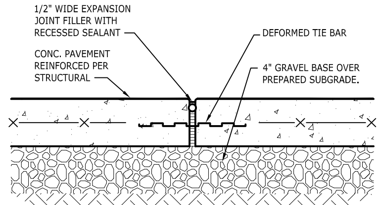
6L EXPANSION JOINT
