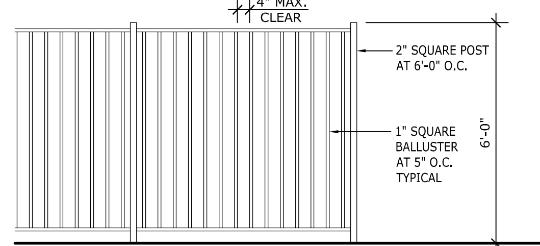
9D TYP. ALUMINUM FENCE ELEV. AS102 scale: 3/8" = 1'-0"
