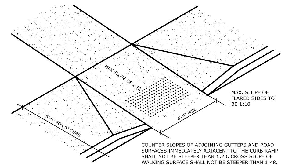
7L RAMP DETAIL AS102 scale: 1/4" = 1'-0"
